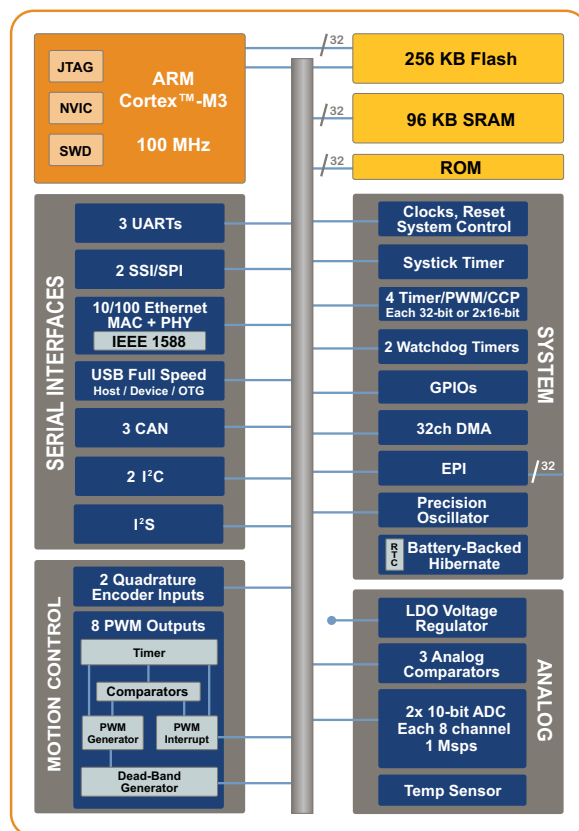
Stellaris Family Block Diagram
