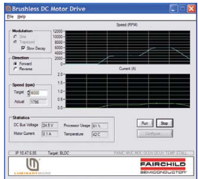
RDK-BLDC Windows Graphical Control Program Screen Shot
